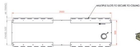
ECO 1000/CE/RP/PC/RX x4 PLATES
