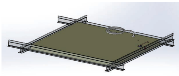
ECO 300/80/FF/RP/PC/RX 595x595mm 'T' Grid
